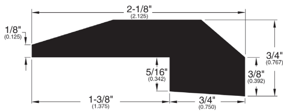
Threshold (008)
