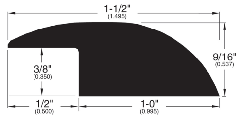
Reducer Overlap (029)
