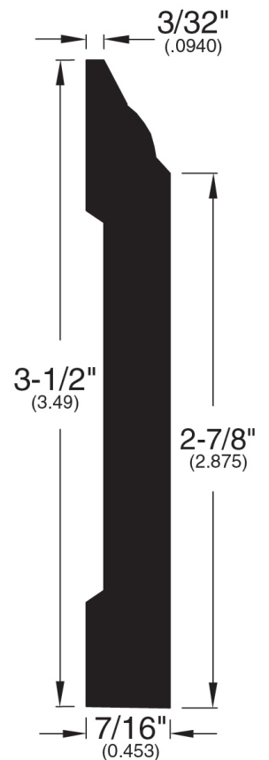
Wall Base (003)
