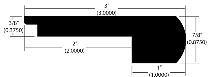
Stair Nose (709)
