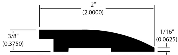
Reducer (707)
