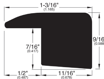
Square Nose (043)
